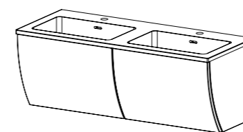
1100 Vanity & Basin D457 x W1110 x H420
