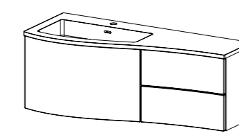
1200 Left Vanity & Basin D480 x W1200 x H420
