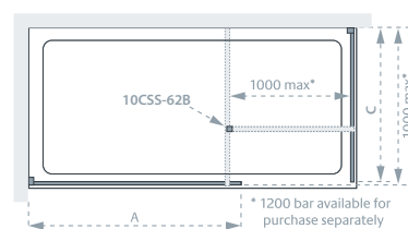
Shower Panel and Side Panel
