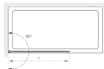
Hinged Shower Panel
