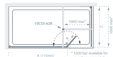
Shower Panel and Bypass Panel and Side Panel
