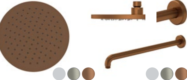
Faber overhead shower Constructed from brass material 250mm(dia) Minimum pressure 0.5bar SVHEAD86 Chrome £225.00 SVHEAD87 Brushed nickel £250.00 SVHEAD88 Brushed bronze £250.00 Faber shower arm Constructed from brass material 74(h) x 414mm(d) SVARM24 Chrome £70.00 SVARM25 Brushed nickel £100.00 SVARM26 Brushed bronze £100.00
